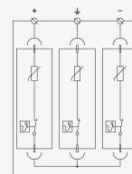
Basic circuit diagram
