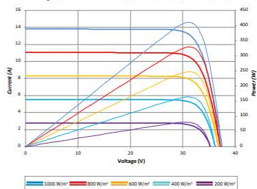
Graphs Current-Voltage & Power-Voltage Curve (410S)
